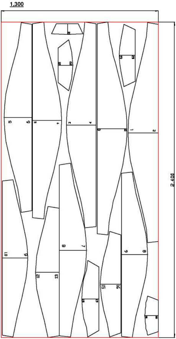
Fig. 5 Positioning of the spiral templates on the steel sheeting for marking and cutting (Segments as indicated)
