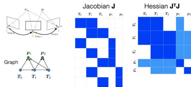
Figure 23.5: Visual SLAM problem with 3 cameras and 2 landmarks (with odometry). Sparsity patterns of the Jacobian and Hessian matrices.
