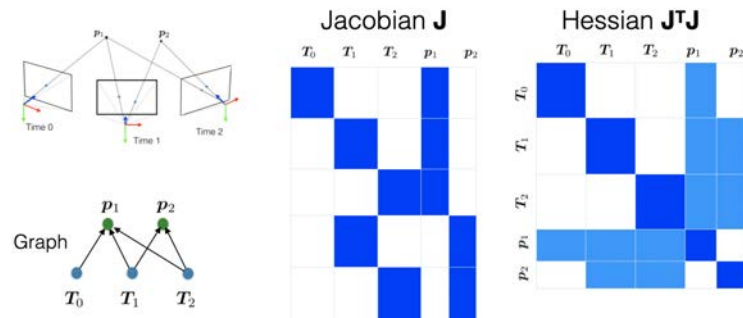
Figure 23.4: Bundle adjustment problem with 3 cameras and 2 landmarks. Sparsity patterns of the Jacobian and Hessian matrices.
