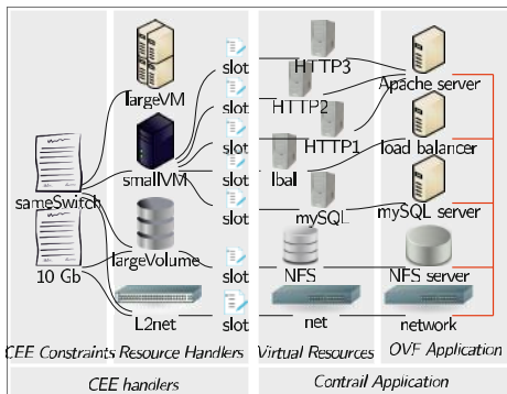
Fig. 4. Constrained Execution Environments and OVF mapping
