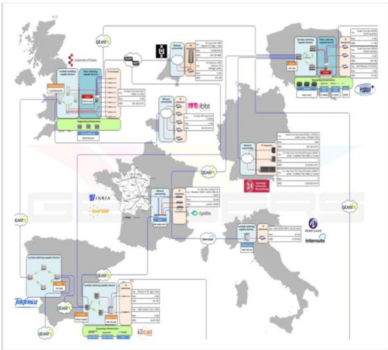
Fig. 2. GEYSERS testbed
