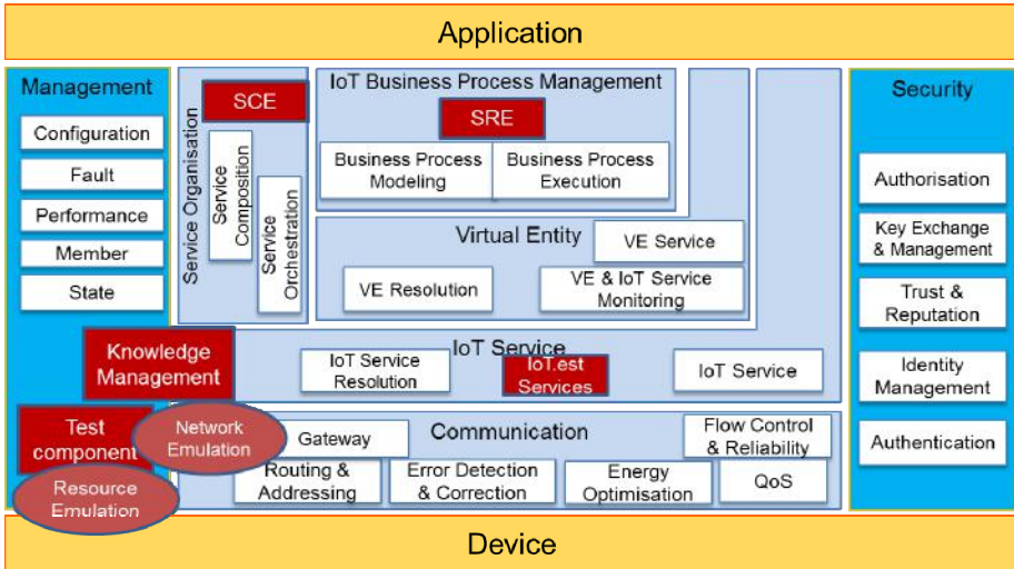
Fig. 2. Mapping of IoT.est functional blocks to IoT-A RA
