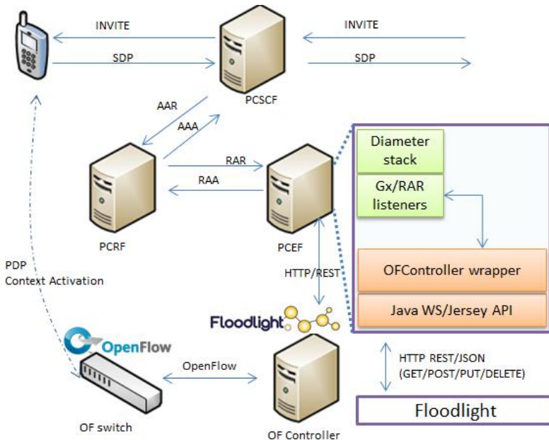
Fig. 2. Openflow integration in OSIMS
