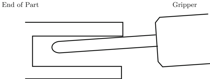
Fig. 2. Gripper construction.
