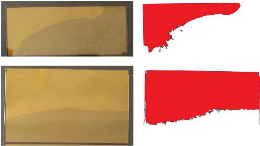
Fig. 11. Image processing applied to peeled samples. ROI (Region of Interest) original image (left) and processed image (right) for calculation of peeled area, in white. Runs reported: 100 A ( a = 10 ; e = 0 ; sample A) on top and 150C ( a = 15 ; e = 0 , sample C) on bottom.
