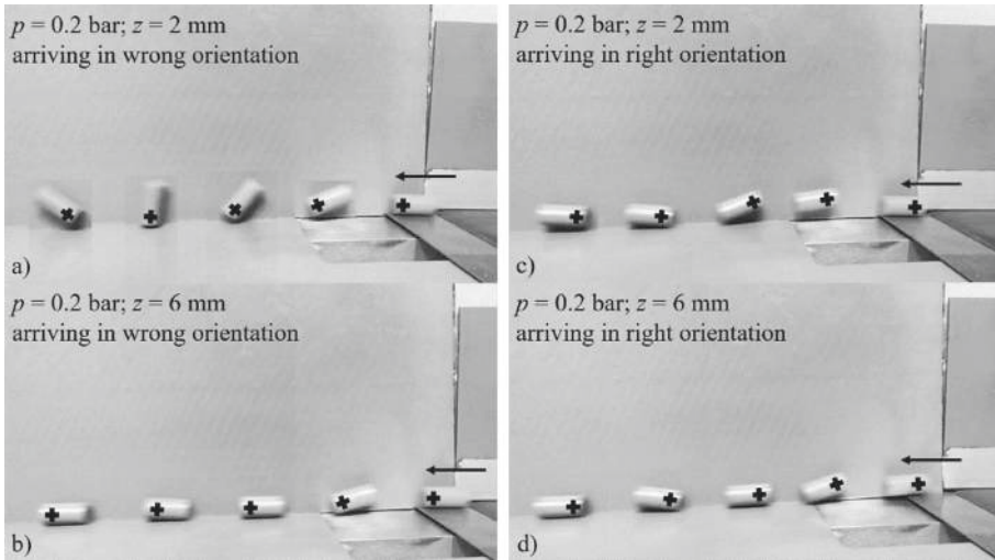
Fig. 8. Trajectories of plastic sleeves with different parameters p and z
