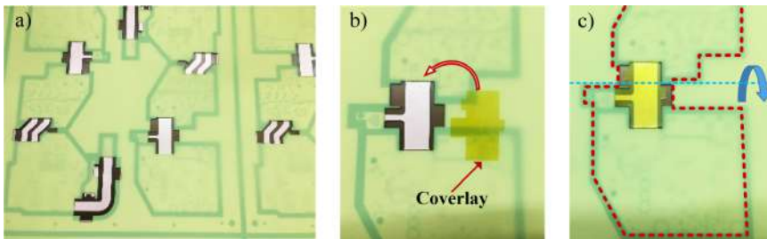
Fig. 3. Coverlay application. Flexible circuit before (a) and after (b) the application of the coverlay. In (c) the red countour highlights the frame to be trimmed out and the blue line indicates the flexion axis of the final device. (Courtesy of Somacis, Italy). (Color figure online)
