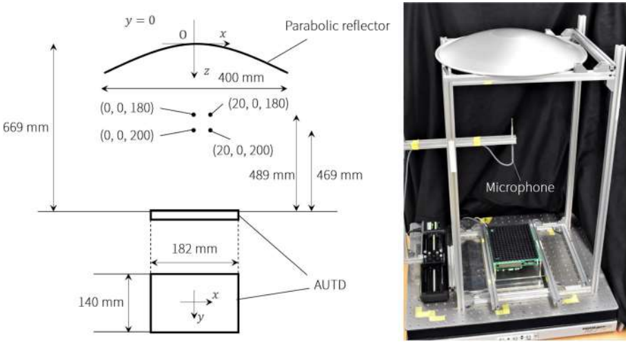
Fig. 2. Geometry of the proposed system. The position (0, 0, 180 mm) is the focus of the reflector.
