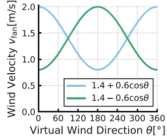
Fig. 3. A Plot of wind velocity
