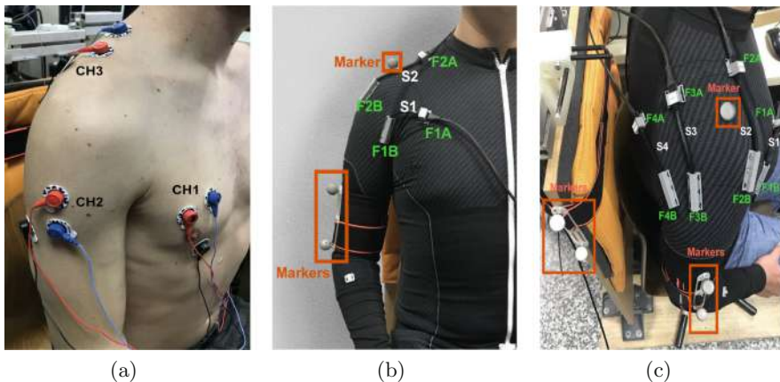
Fig. 1. Soft Sensor Device. sEMG location (1a): Trapezius Descendens (CH3), Deltoides Medius (CH2) and Pectoralis major (CH1). Markers location: one over the shoulder Acromion bone, two on the arm (1b) and two vertically over the base (1c).
