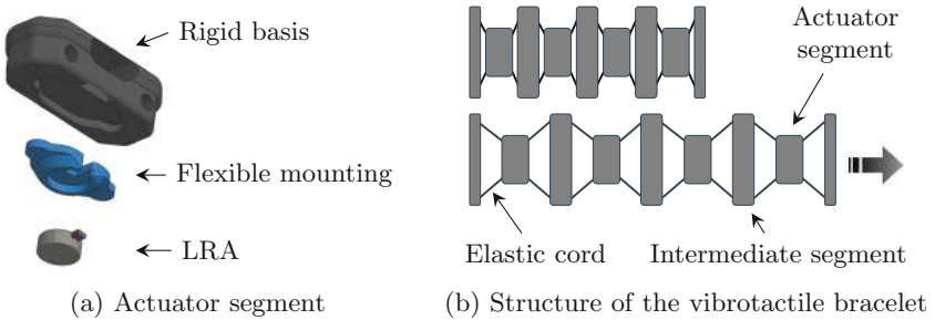
Fig. 2. Each actuator segment consists of a rigid basis, a flexible mounting, and an LRA (a). Actuator segments and intermediate segments are arranged alternating on an elastic cord (b). The zigzag pattern of the elastic cord ensures equal distances between the actuators in relaxed and stretched state [12].
