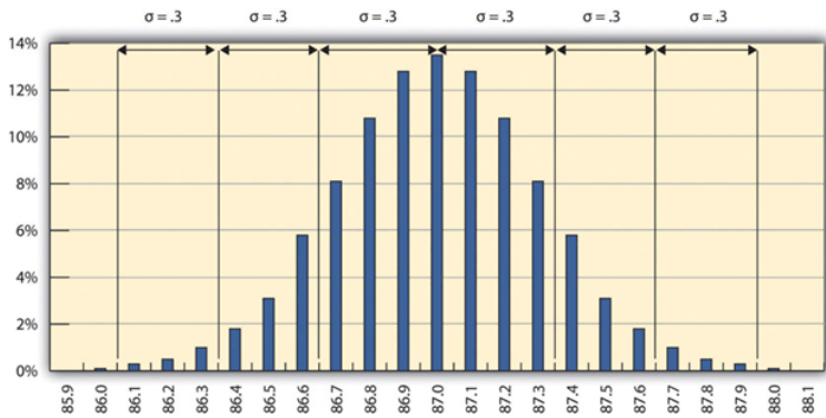
Figure 10.3 The 68-95-99.7 Rule
