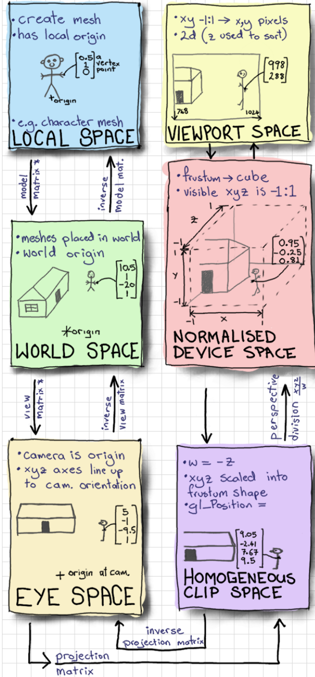
Figure 13.1: Transformation Pipeline
