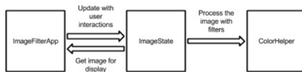
Figure 11.5: Architecture diagram
