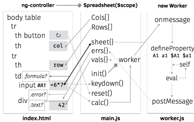
Figure 19.7: Architecture Diagram
