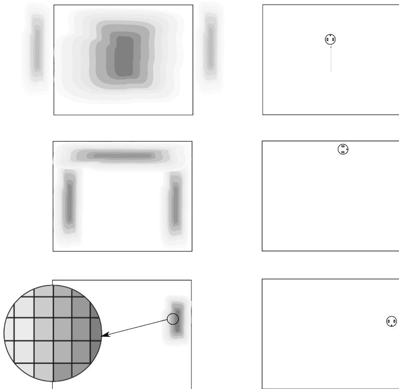
Figure 9.3.: Markov localization on a grid. The left column shows the likelihood to be in a specific cell as grey value (dark colors correspond to high likelihoods). The right column shows the actual robot location. Arrows indicate previous motion. Initially, the position of the robot is unknown, but recorded upwards motion makes positions at the top of the map more likely. After the robot has encountered a wall, positions away from walls become unlikely. After rightwards and down motions, the possible positions have shrunk to a small area.
