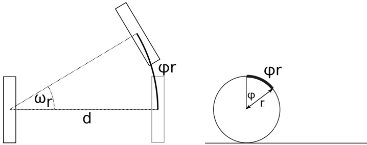
Figure 3.7.: Left: Differential wheel robot pivoting around its left wheel. Right: A wheel with radius r moves by \phi r when rotated by \phi degrees.
