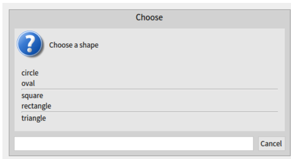
Figure 12-40 Pop-up menu.
