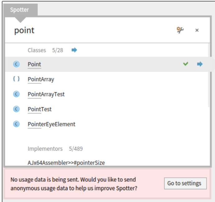
Figure 2-17 Opening Spotter
