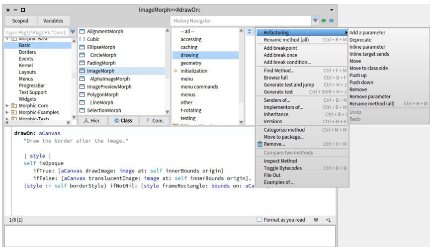
Figure 7-14 Refactoring operations.
