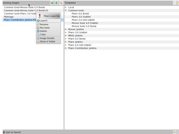
Figure 2-5 PharoLauncher - GUI
