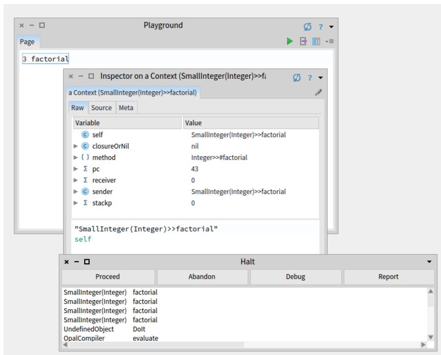
Figure 14-8 Inspecting thisContext.
