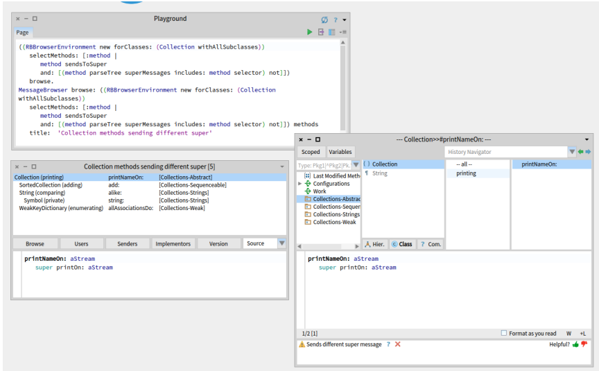
Figure 14-7 Finding methods
