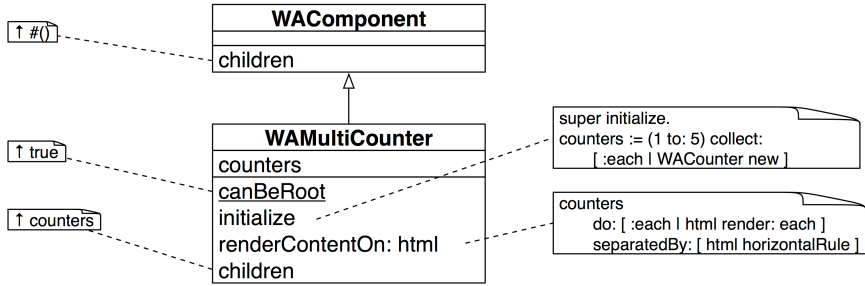
Figure 13-12 WAMultiCounter.
