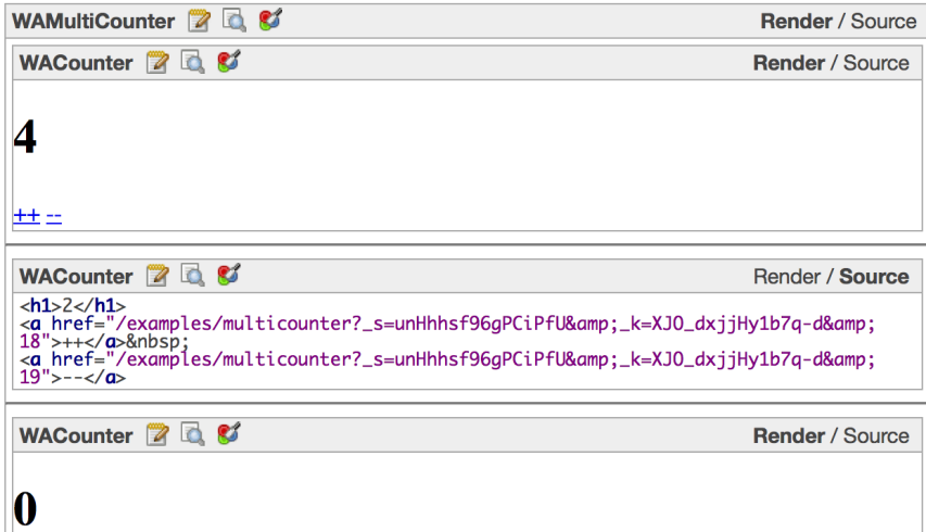
Figure 13-7 Independent subcomponents.
