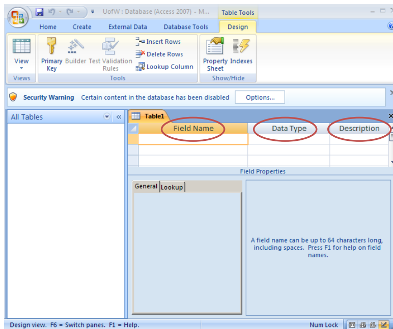
Figure 2.4 Table Design View
