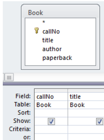
Figure 4.9 Query showing specific fields
