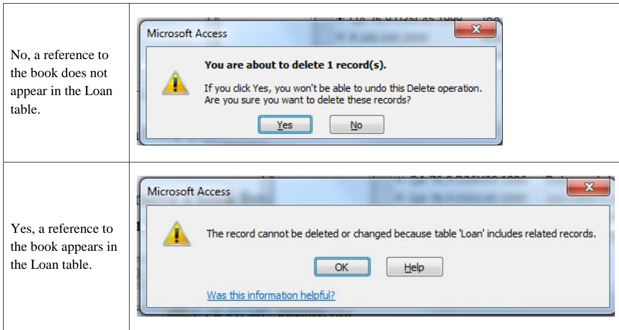
Figure 1.12 Attempting to delete a row
