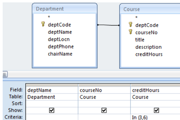
Figure 6.23 Query with required fields
