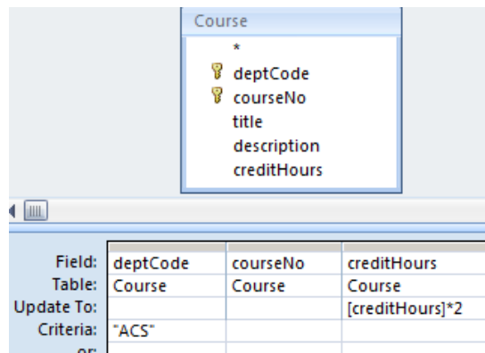
Figure 6.29 Update query with Update To line
