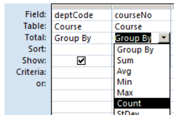
Figure 6.20 Step 3: Choose the appropriate aggregate for the group
