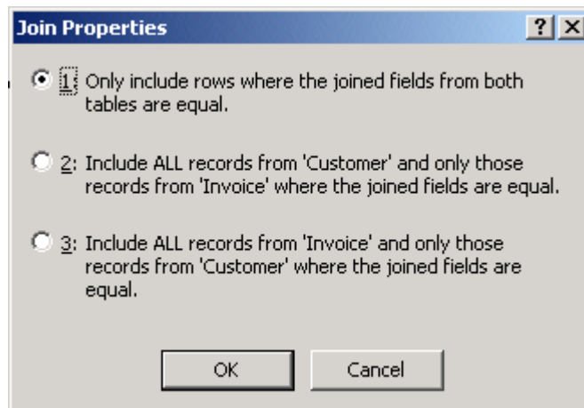
Figure 6.32 Choosing inner join or outer join
