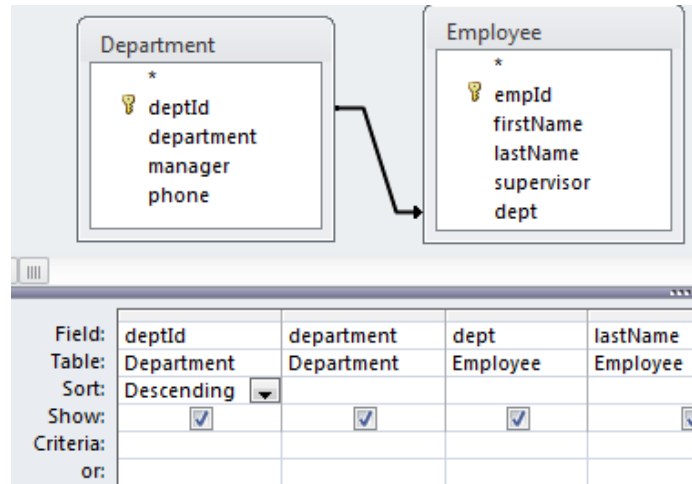
Figure 6.38 Outer join – all rows of Department
