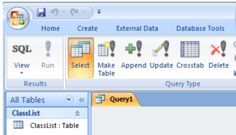
Figure 9.2 Choose SQL view for the query
