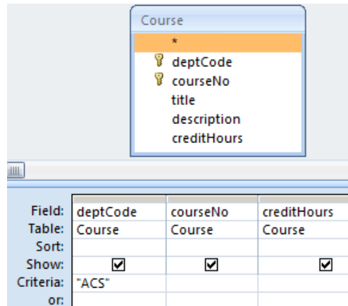
Figure 6.28 Simple select query
