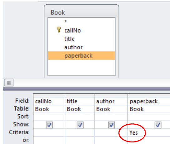
Figure 4.10 Query with selection criteria
