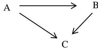
Figure 10.9 Non-key attributes and a transitive dependency
