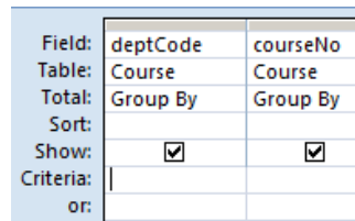
Figure 6.19 Step 2: Total line is added to the grid
