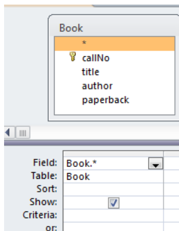
Figure 4.4 Choosing all fields of the table
