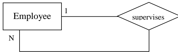
Figure 7.24 Recursive relationship involving Employee twice
