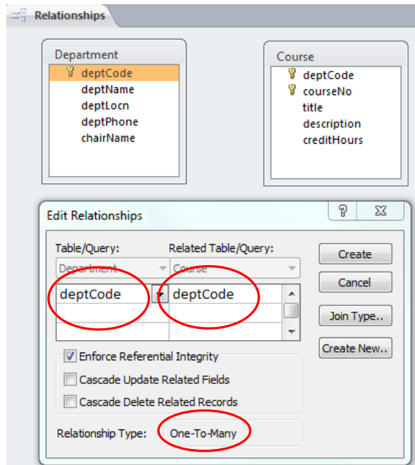
Figure 5.4 Defining a one-to-many relationship
