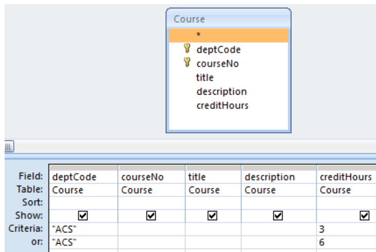
Figure 6.2 Two expressions that are ORed
