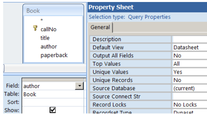
Figure 6.14 Setting Unique Value to yes
