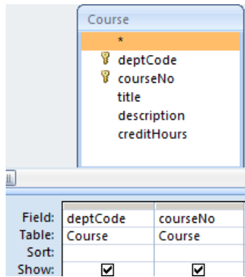
Figure 6.18 Step 1: the fields needed
