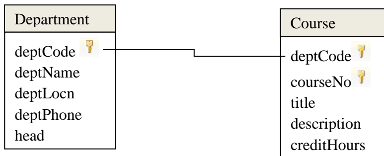
Figure 5.1 Showing a relationship between two tables
