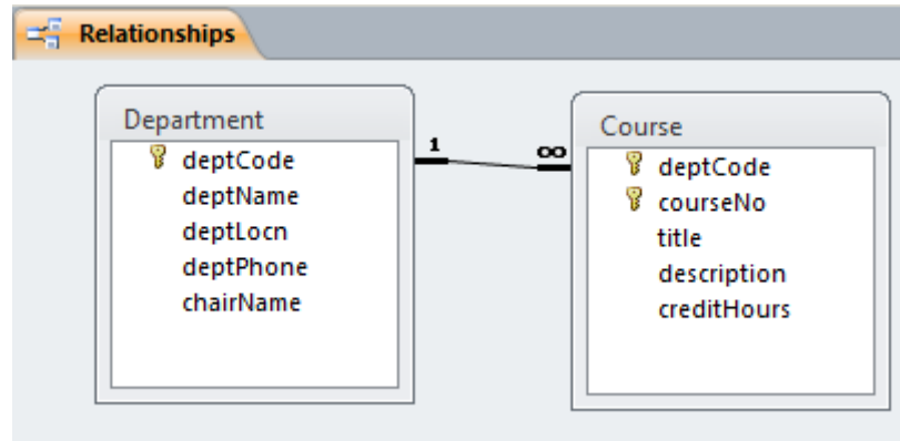
Figure 5.3 Relationship: department offers courses
