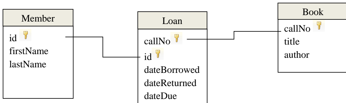
Figure 5.2 Showing relationships involving three tables
