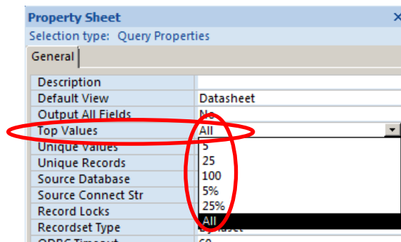
Figure 6.9 Setting the Top Values property
