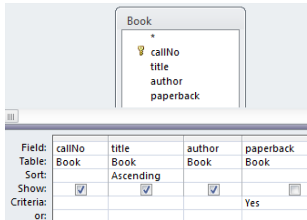
Figure 4.12 Query results can be sorted
