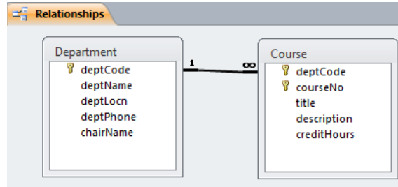
Figure 5.5 One-to-many relationship: department offers courses
