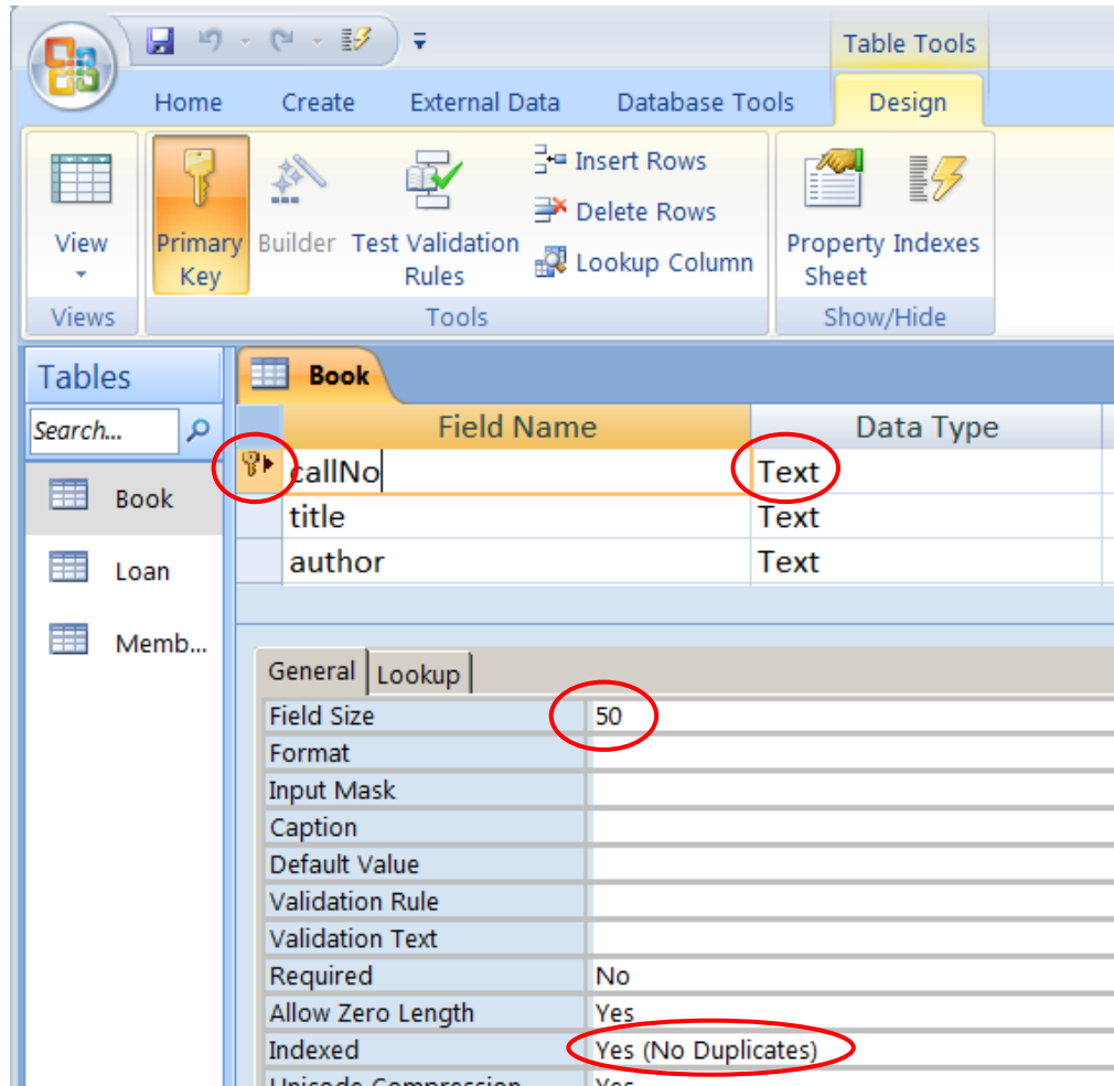
Figure 1.14 Table Design View
