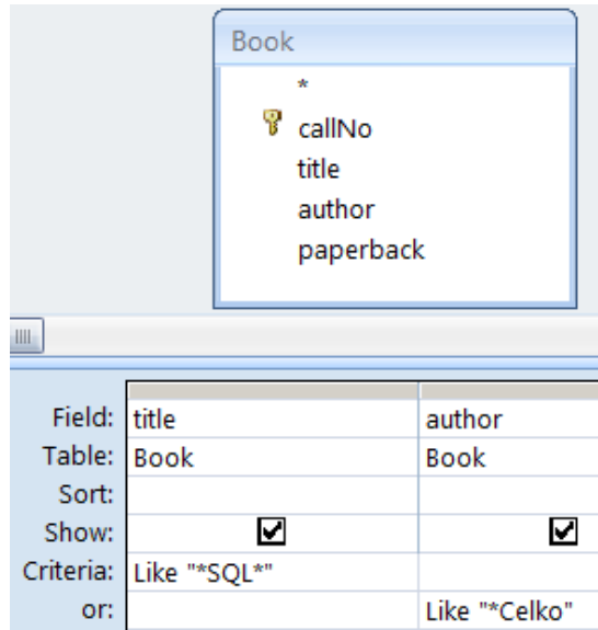
Figure 4.14 Criteria on different criteria lines are ORed
