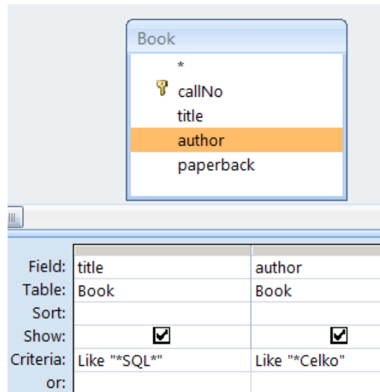
Figure 4.13 Criteria on one criteria line are ANDED
